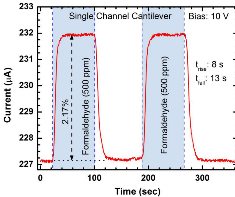
Figure 4.7 Response of a SC- TMH sensor to 500 ppm of formaldehyde at 10 V dc bias. Current magnitude changed by 2.17% with rise time and fall time of 8 s and 13 s respectively. Two sensing cycles are shown here to demonstrate repeatability.
